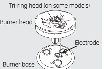
Make sure the ring in the burner head is positioned over the electrode and that the burner head is fully inserted inside the burner base. A small gap between the base and head is normal.
